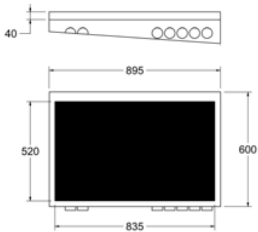
HOB DETAIL
