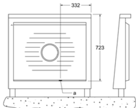
CONNECTIONS DETAIL
